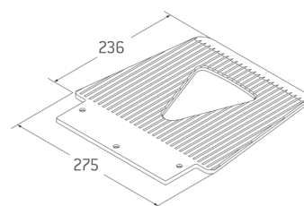
Schaufel Standard
